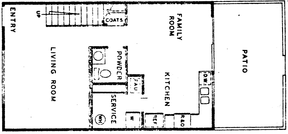
LOWER FLOOR
