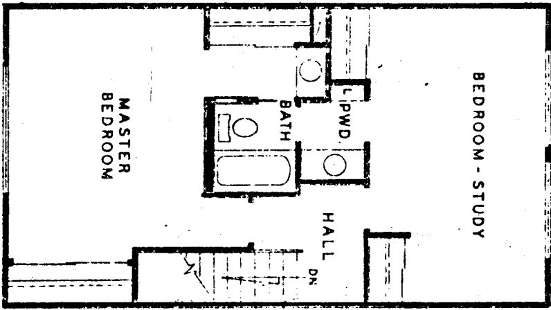
UPPER FLOOR
