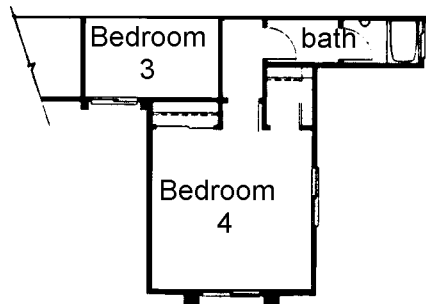
Optional configuration - elevations B & D
