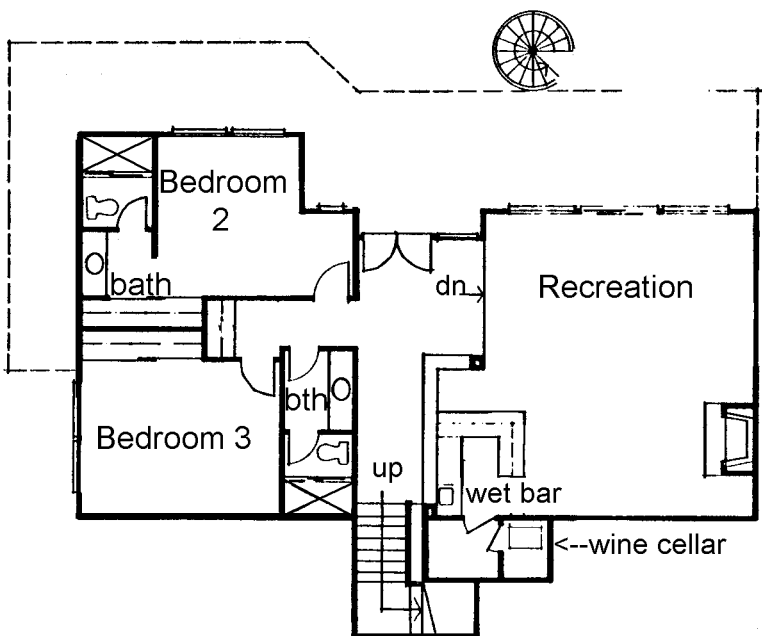
Lower Level
