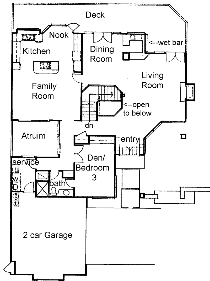
Upper Level
