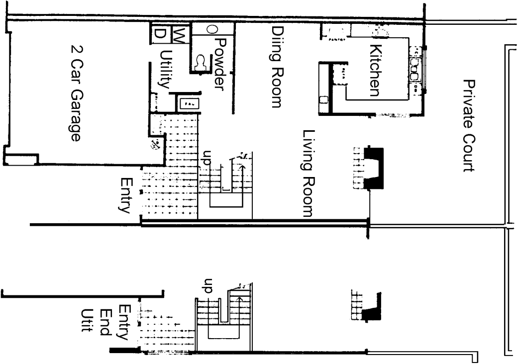
First Floor
