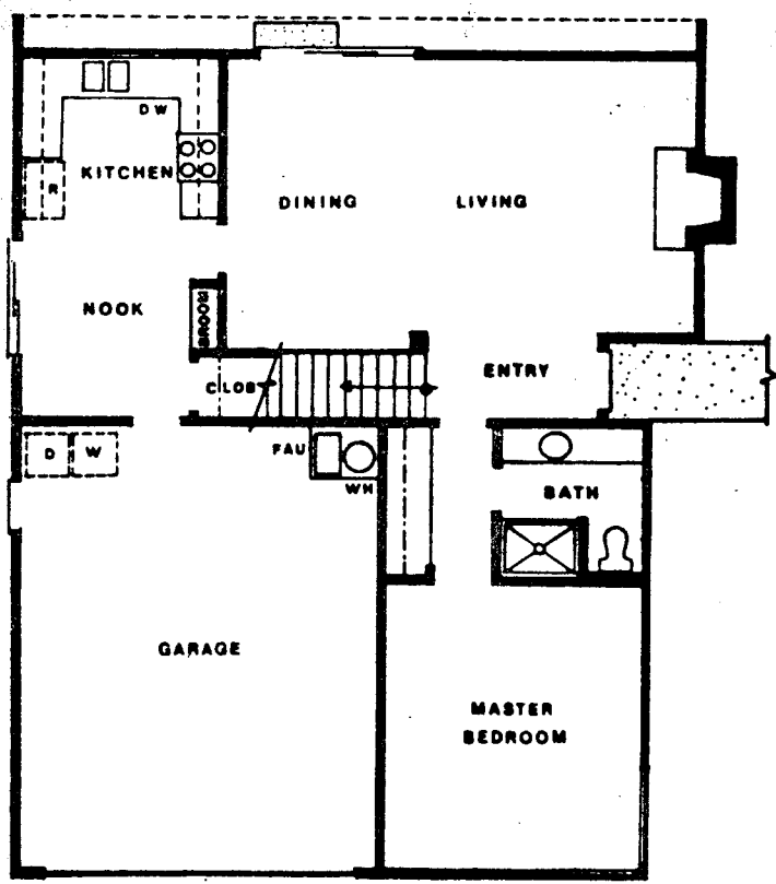
FIRST FLOOR PLAN NO. 09
