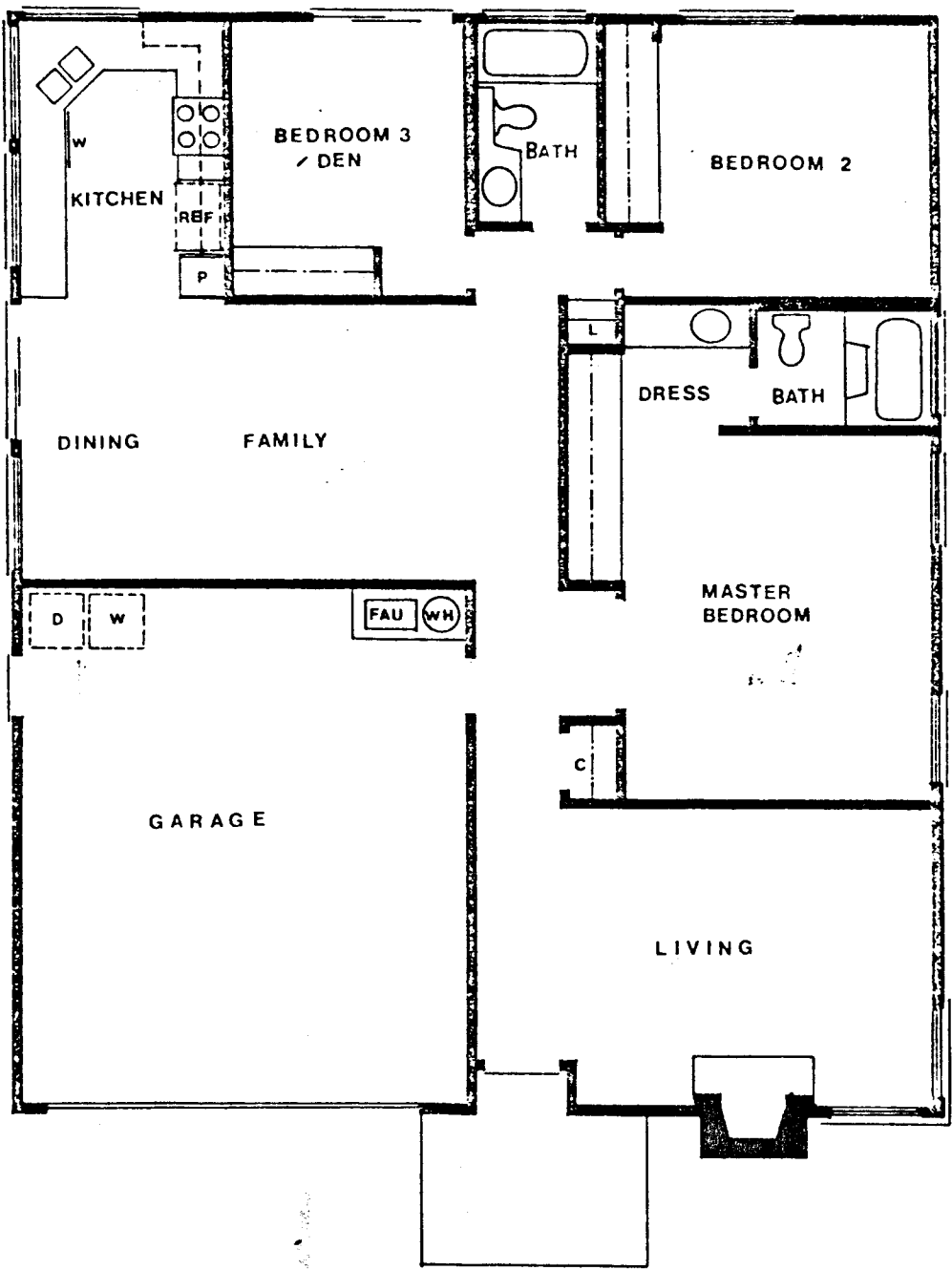
FLOOR PLAN NO 11
