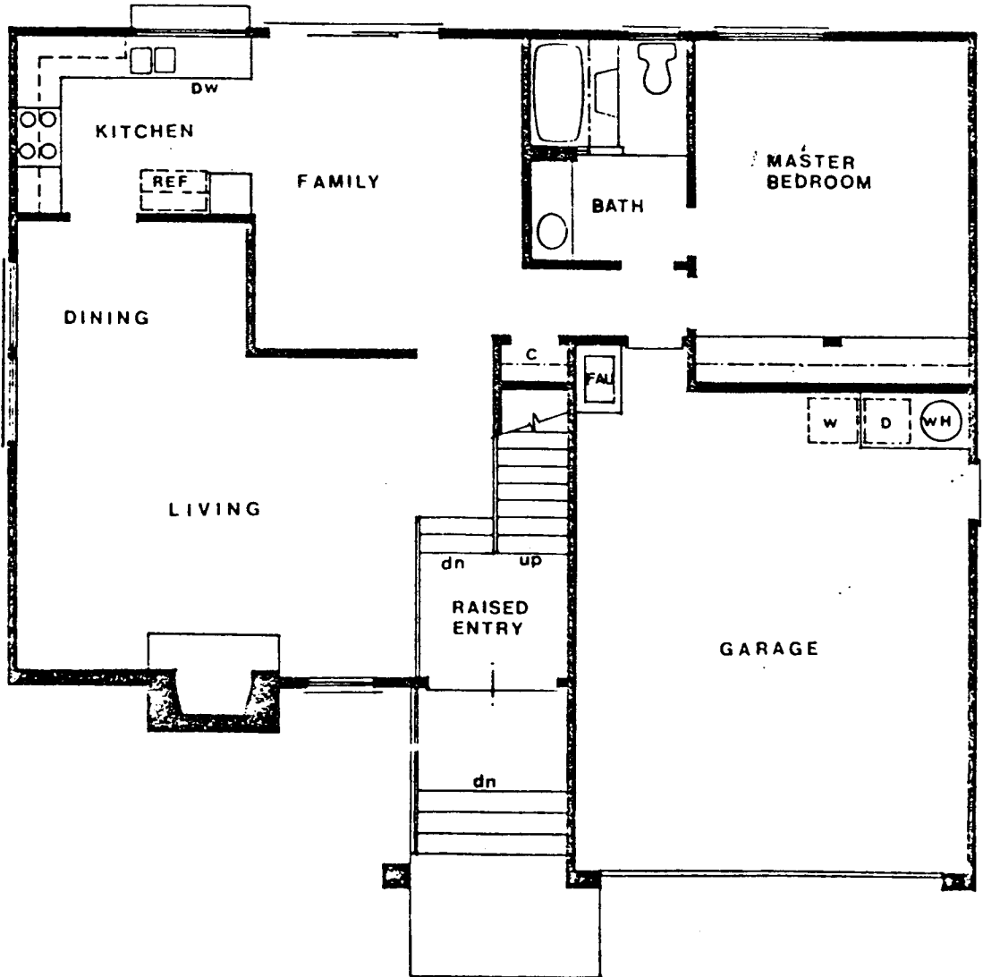
FIRST FLOOR PLAN 80
